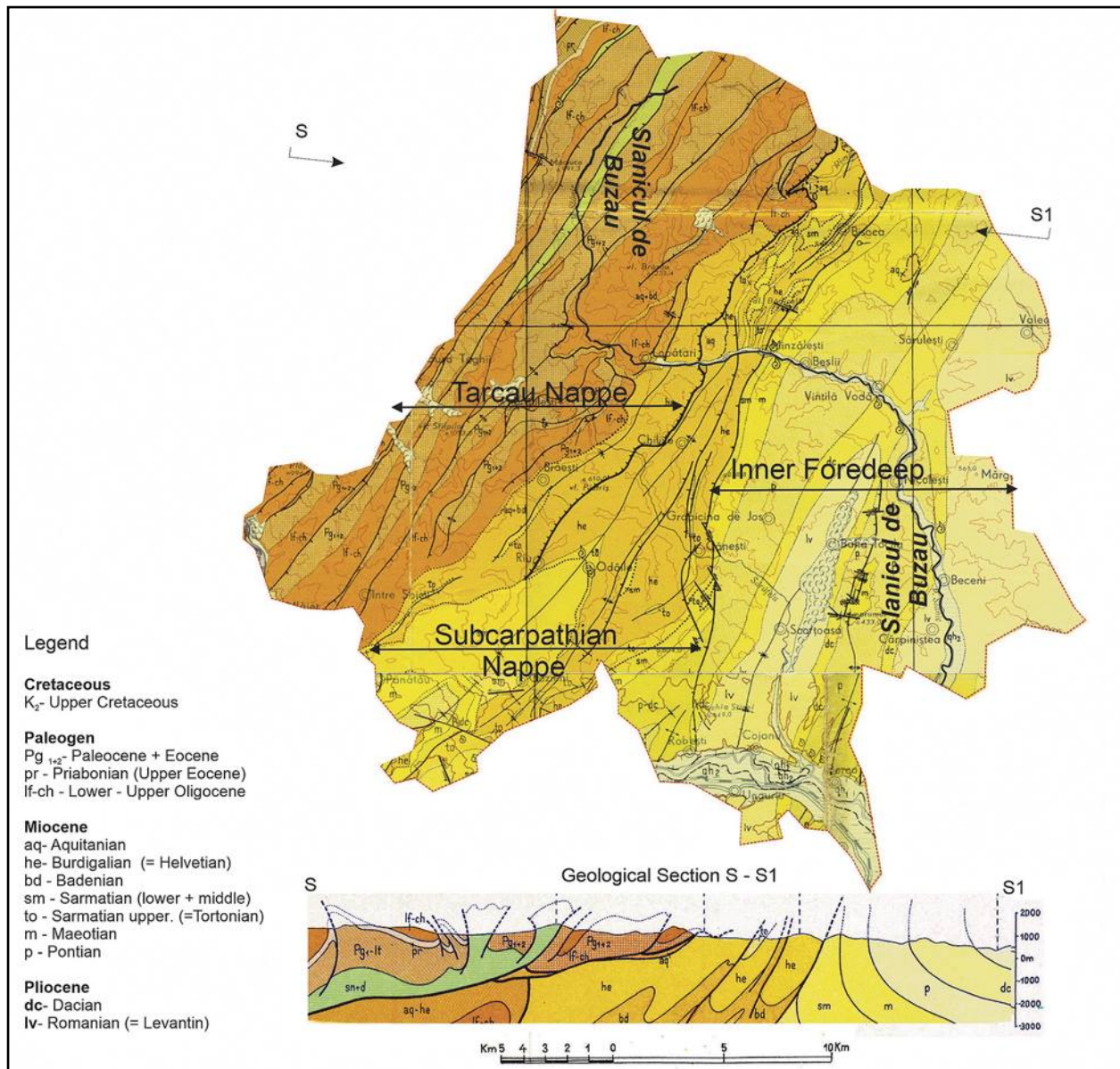
Fig. 3. Geological map of the Buzău Land Geopark that includes the region crossed by Slănicul de Buzău river (after map Motaș et al. , 1967 and Murgeanu et al. , 1968, Maps scale 1:200,000 Sheets Covasna and Ploiești, published by the Geological Institute of Romania).
