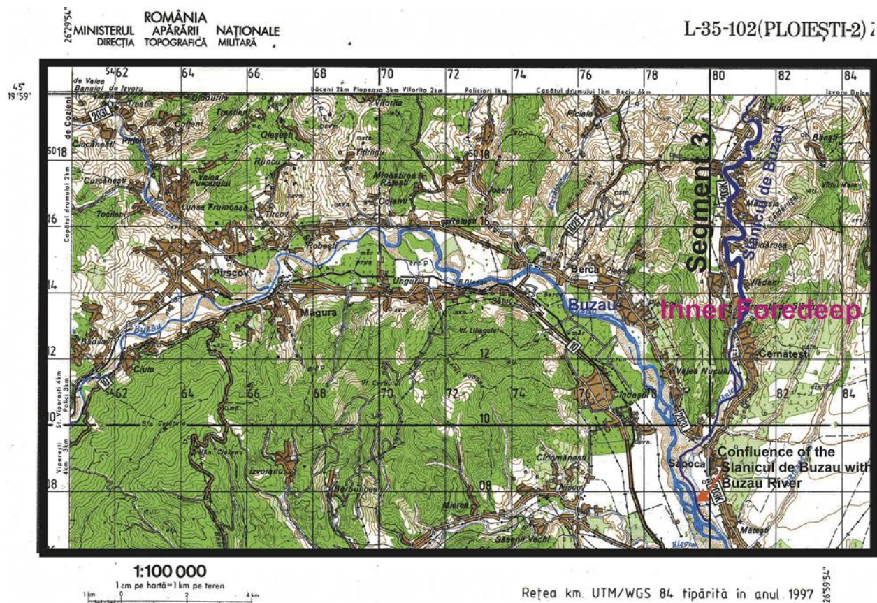
Fig. 13. Segment 3 of the Slănicul de Buzău, showing a flow direction N-S, and including the confluence with the Buzău River at Săpoca.
