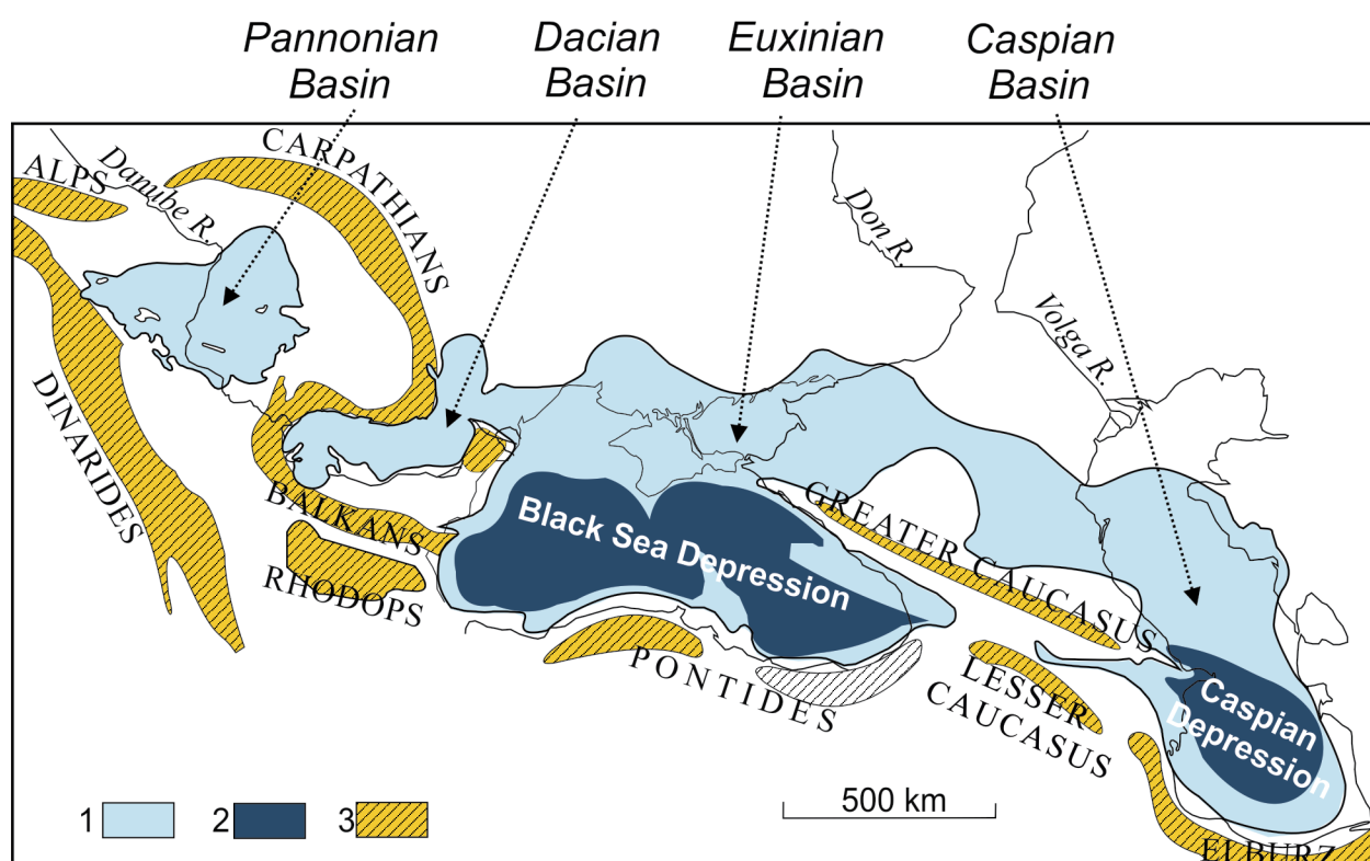
Fig. 3. Paratethys Domain during the Early Maeotian. Simplified, from Popov et al. (2004).
