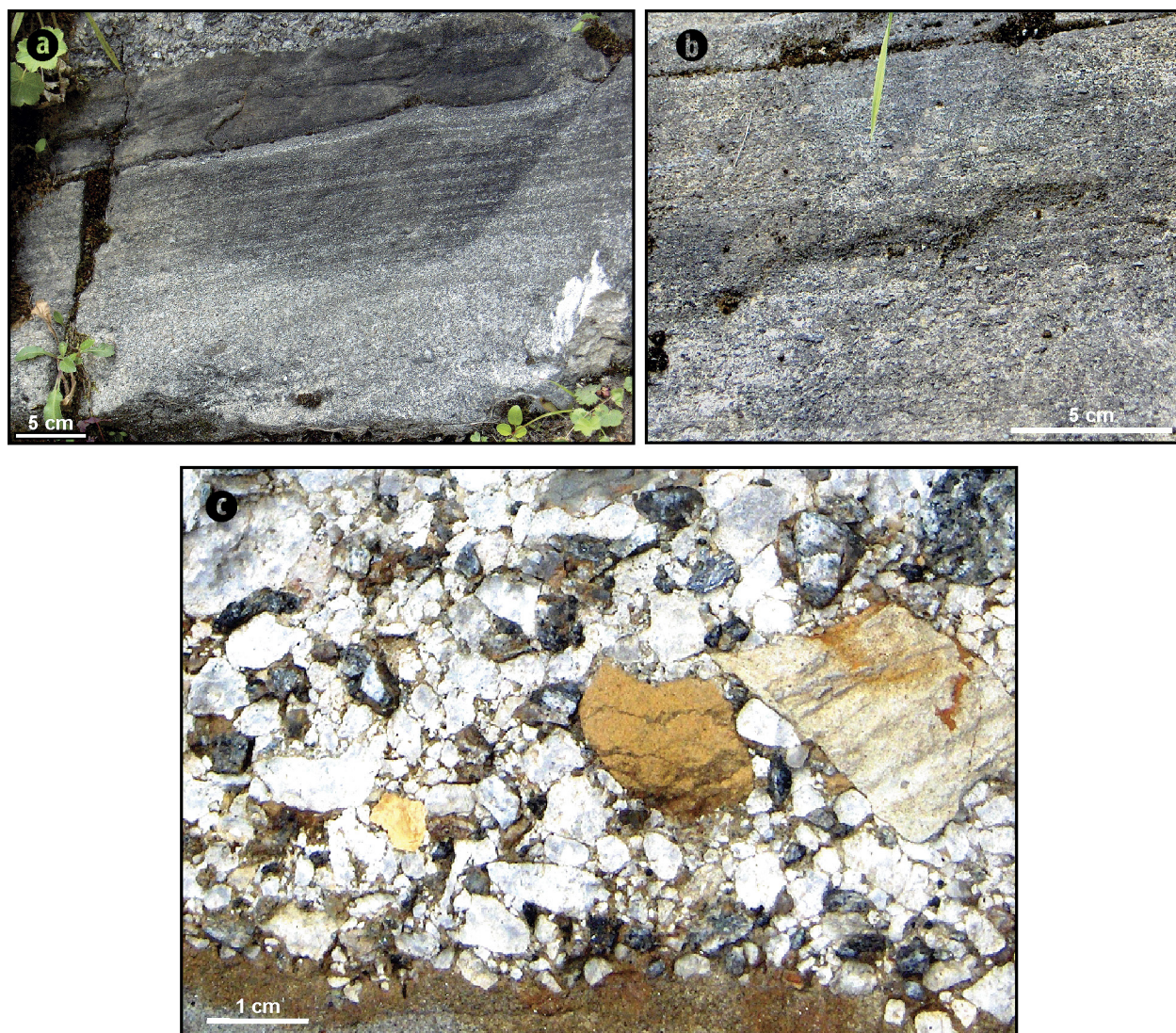
Fig. 8. Răciu Breccia with normal grading and parallel lamination. Images (b) and (c) show details from the upper and lower parts of the graded layer (a), respectively. Jepsi River, Bușteni town.
