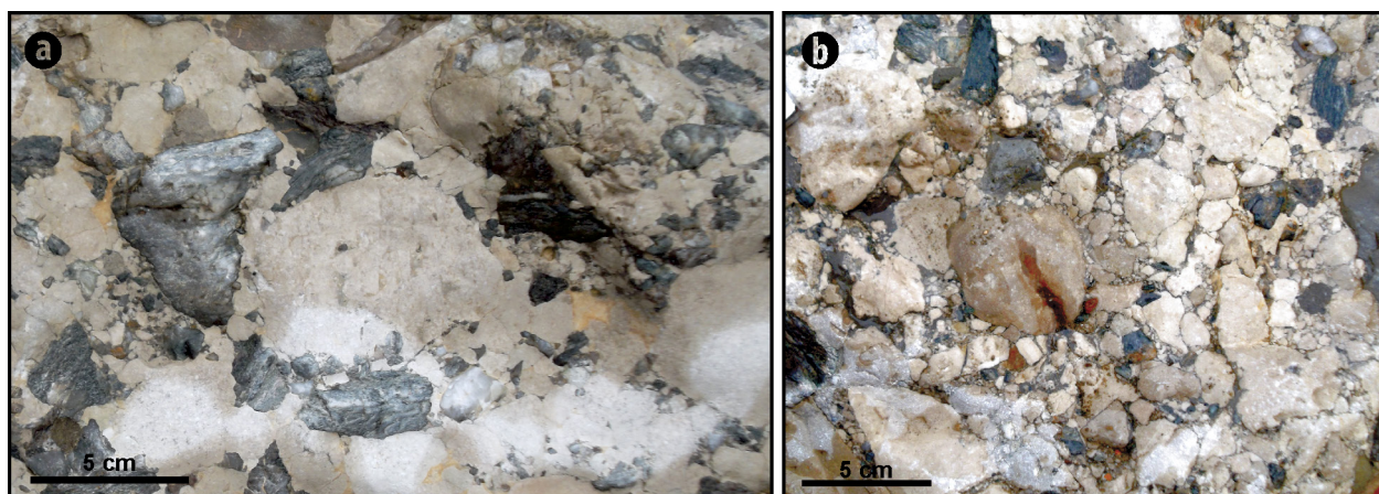
Fig. 9. Matrix in Răciu Breccia. (a) Răciu Breccia without matrix, with interlocked limestone clasts. (b) Răciu Breccia with matrix. Ialomița River, downstream from the confluence with Gâlmei River.
