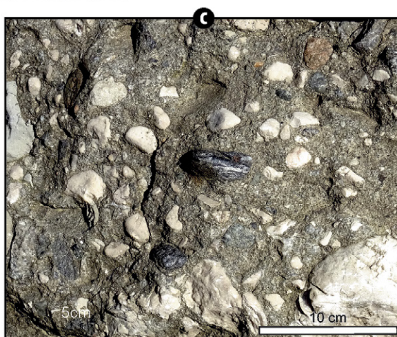
◄ Fig. 14. Conglomerate interbeds in the medium- and coarse-grained sandstone facies. (a) Very fine-grained conglomerate intercalation. Coman River. (b) Conglomerate with dominant metamorphic rock clasts. Coman River. (c) Fine-grained conglomerate with dominant limestone clasts. Chiliilor River.
