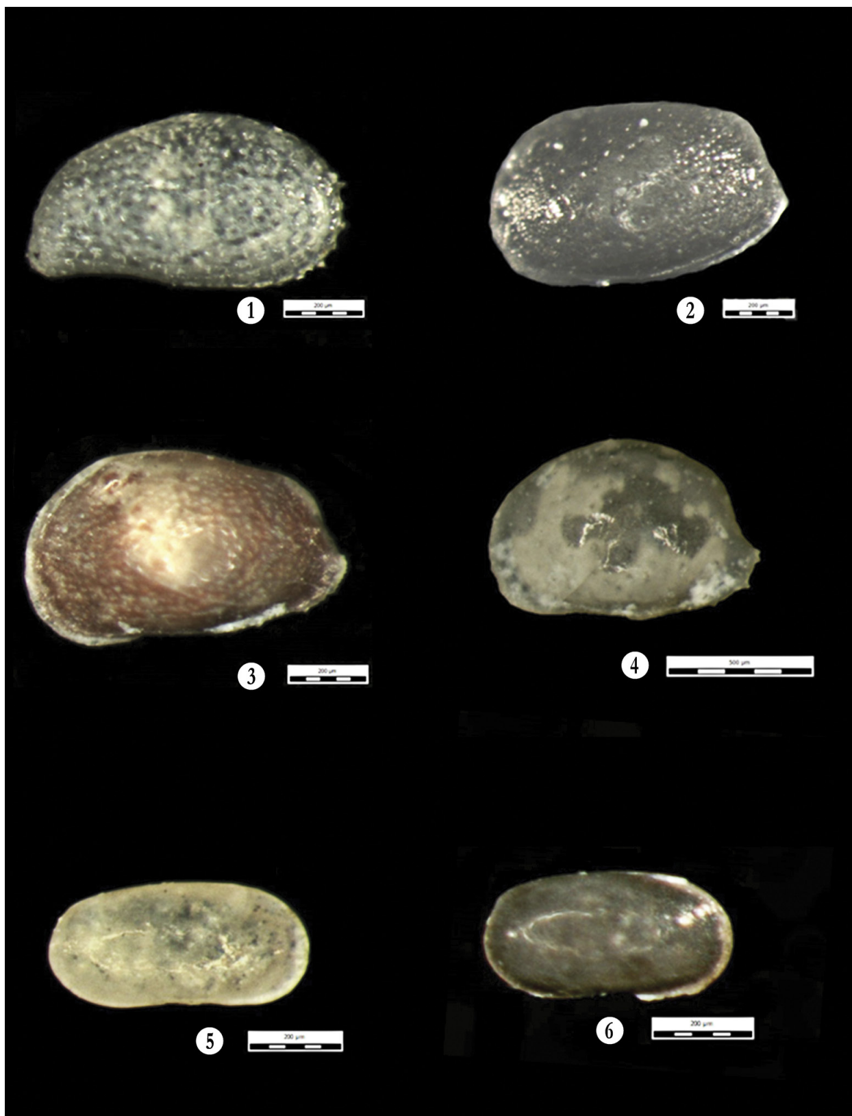
Plate 3. Völnynian ostracods from Blejești area. All valves are in external lateral view. LV = left valve, RV = right valve. 1. Cytheridea hungarica (Zalányi) – RV, 2. Aurila mehesi (Zalányi) – with pyritized, LV, 3. Aurila mehesi (Zalányi) – LV, 4. Aurila merita (Zalányi) – LV, 5. Amnicythère tenuis (Reuss) – RV, 6. Amnicythère tenuis (Reuss) – infilled with pyrite, RV.
